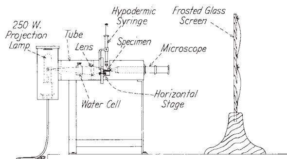
FIG. 1 Projection Apparatus
